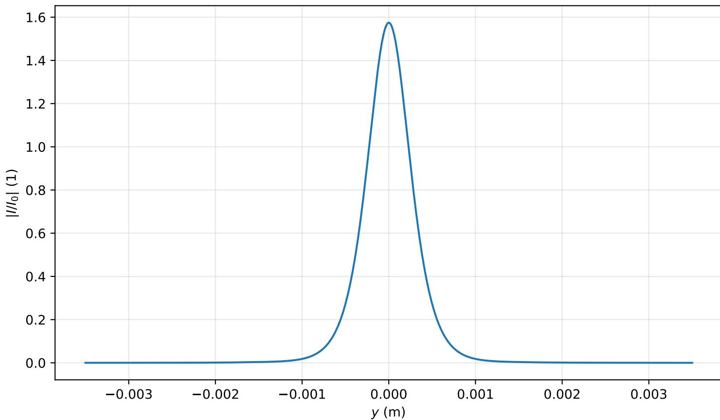
Intensity profile I(x=0, y, z=2.946)/I_0 , \text{Pin}=0.9\text{Pcr} , artificial time
